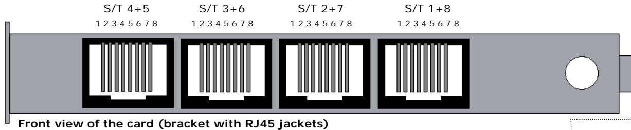
Front view of the card (bracket with RJ45 jackets)
